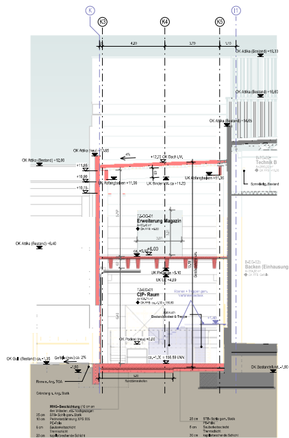
TZ_SCHN_Quer 02
