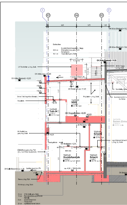
TZ_SCHN_Quer 01
