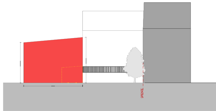
West 1:100
